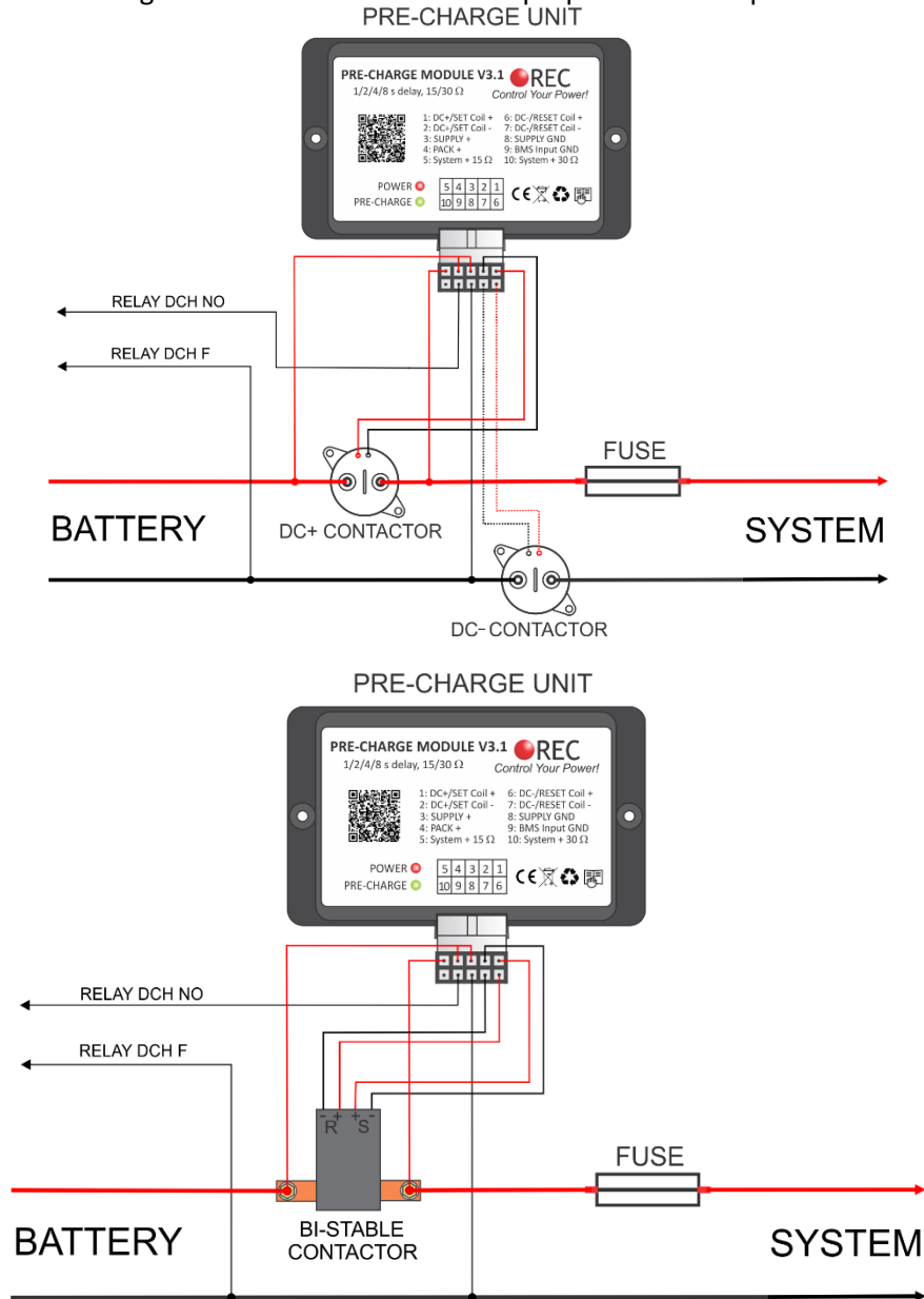
Figure 11: Contactor – Pre-charge module connection schematics with battery voltage contactor drive.
