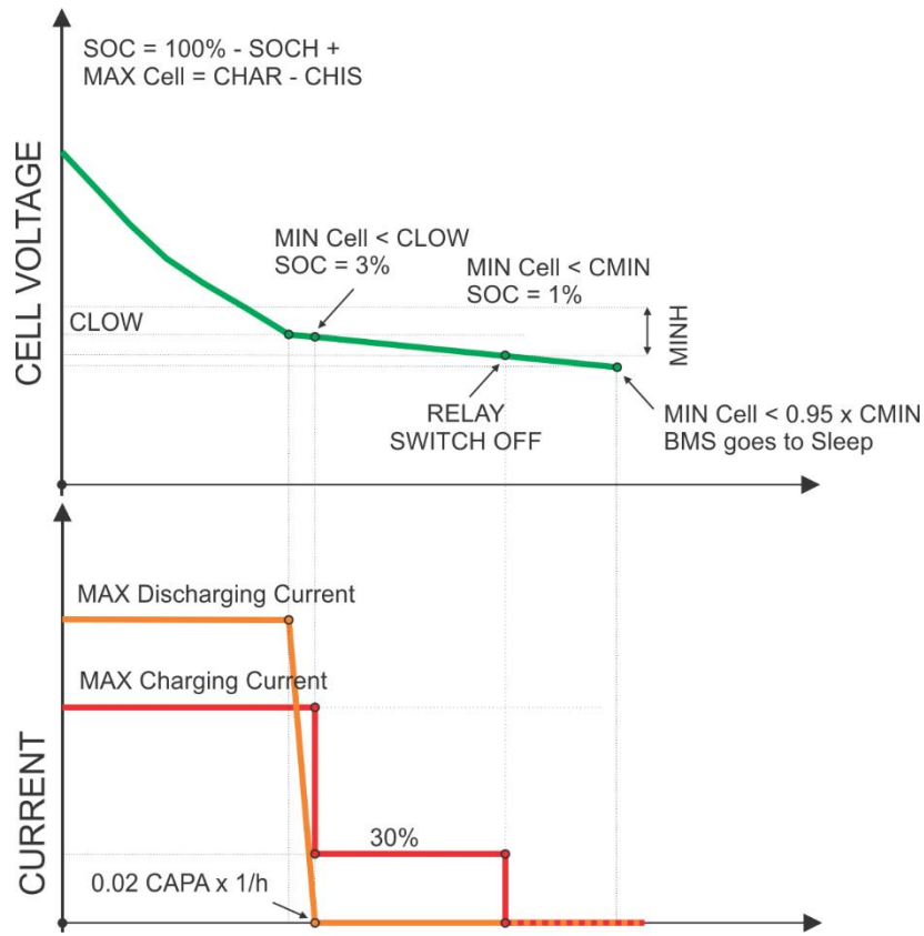
Figure 9: Discharging diagram
