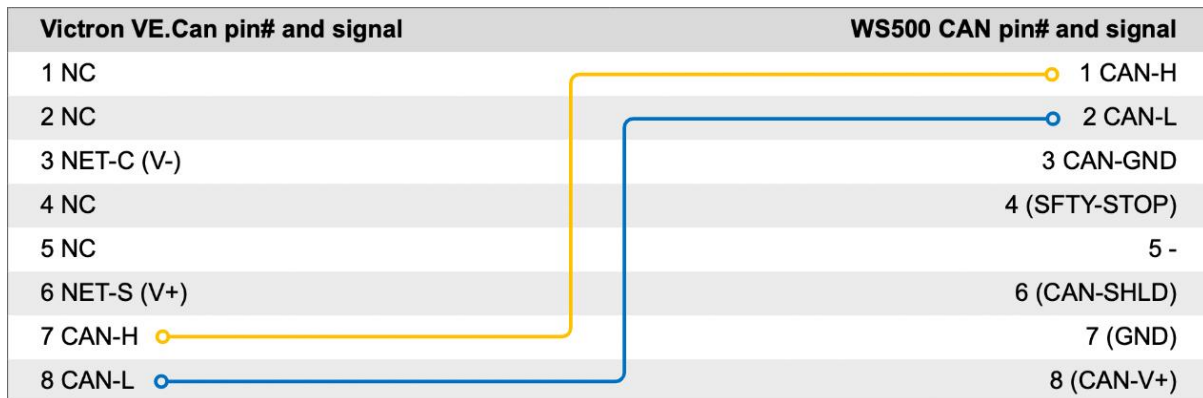
Figure 6: Wakespeed CAN RJ45 pinout.
