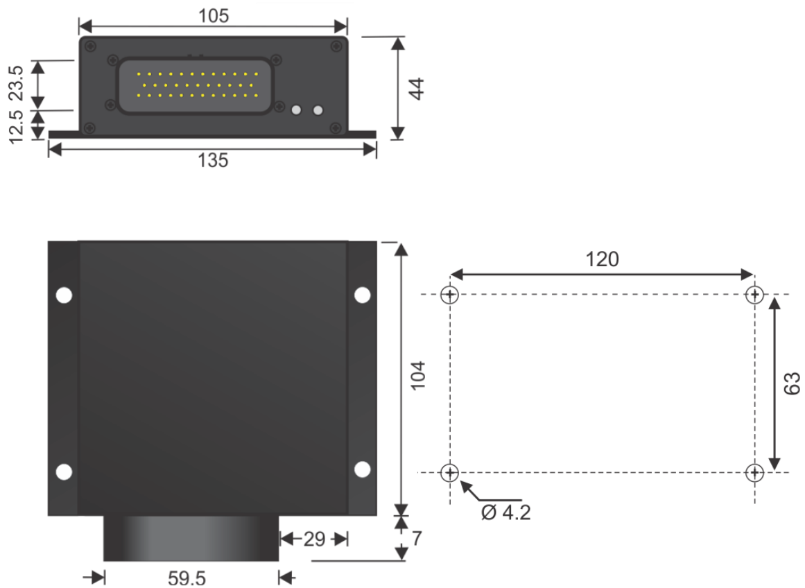
Figure 13: BMS dimensions.
