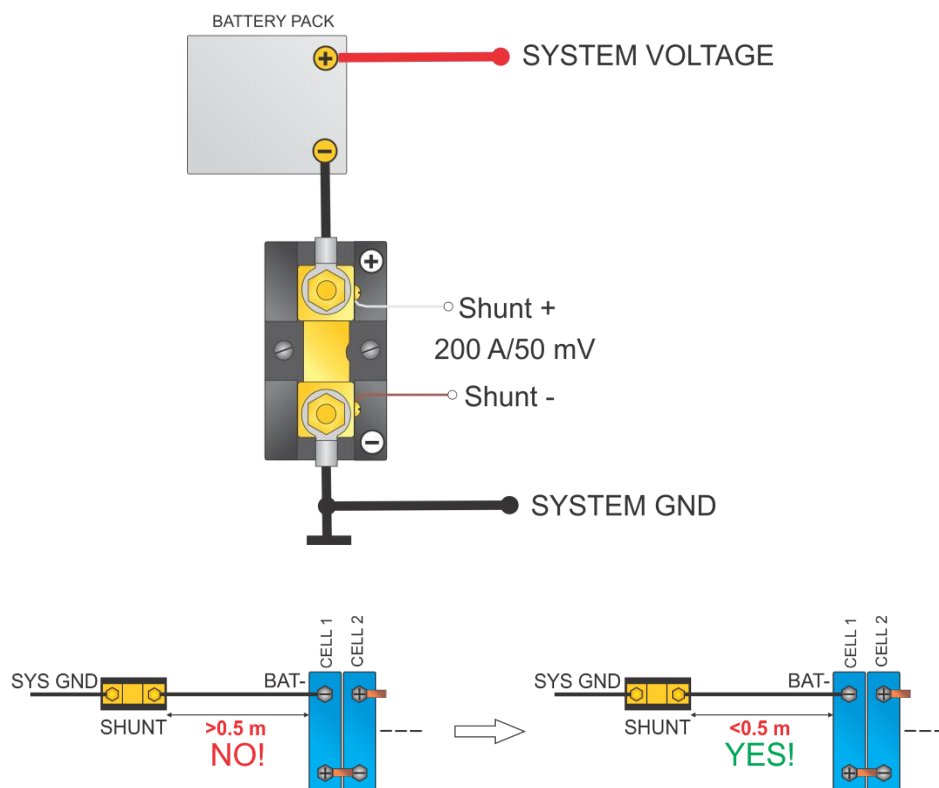
Figure 7: Shunt resistor connection.
