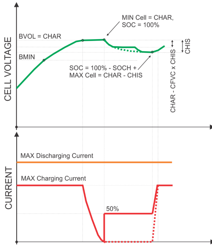
Figure 8: Charging diagram
