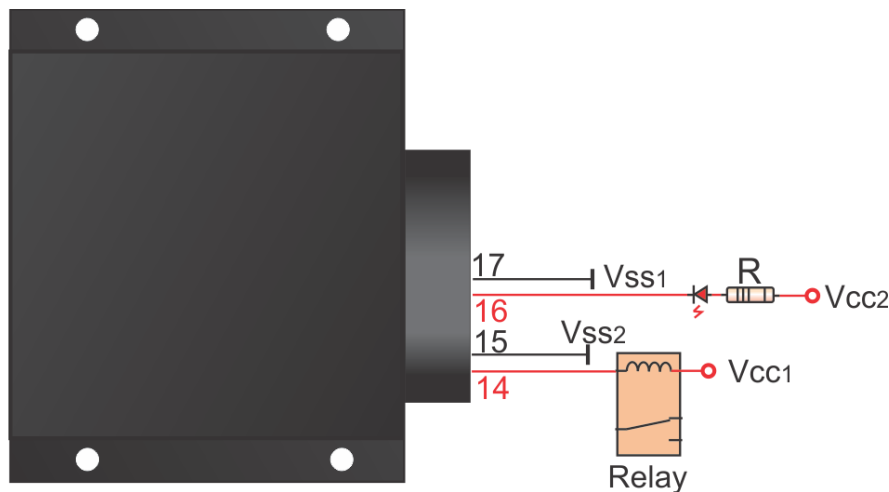
Figure 10: BMS digital outputs schematics.
