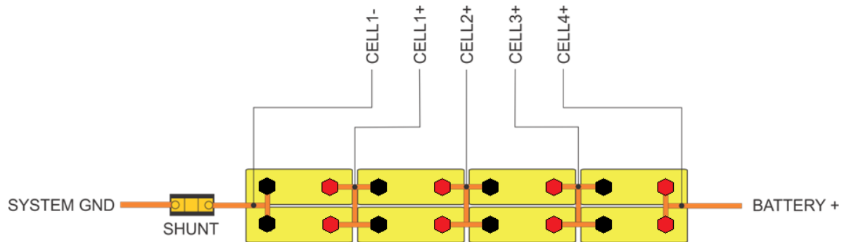
Figure 12: 2P4S battery pack connection.
