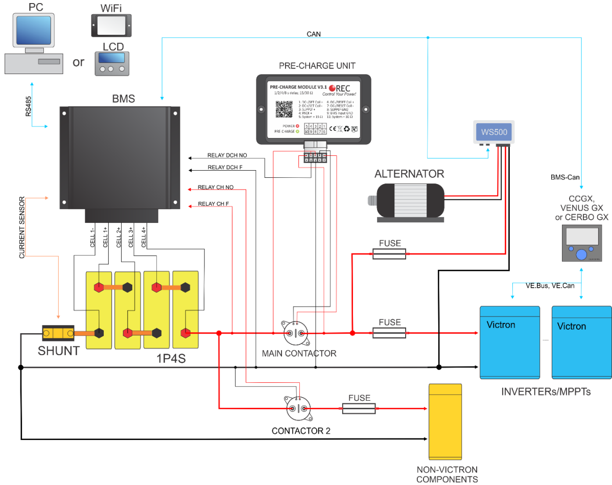
Figure 1: System overview.
