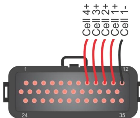
Figure 3: Battery pack connection plug – wiring side.
